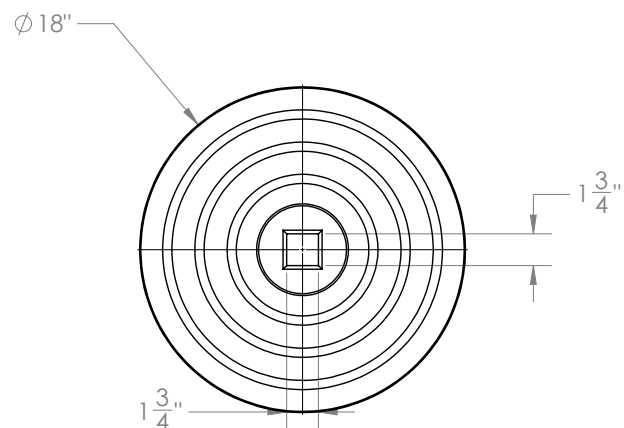
Square Hole Sign Base
