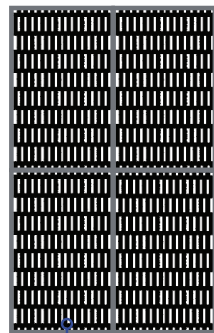
20' W x 30' L Using (2) 10' x 14' Mats and (2) 10' x 16' Mats Total coverage: 616 sq. ft.
