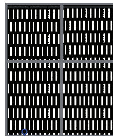
24' W x 30' L Using (2) 12' x 16' Mats and (2) 12' x 14' Mats Total coverage: 740 sq. ft.
